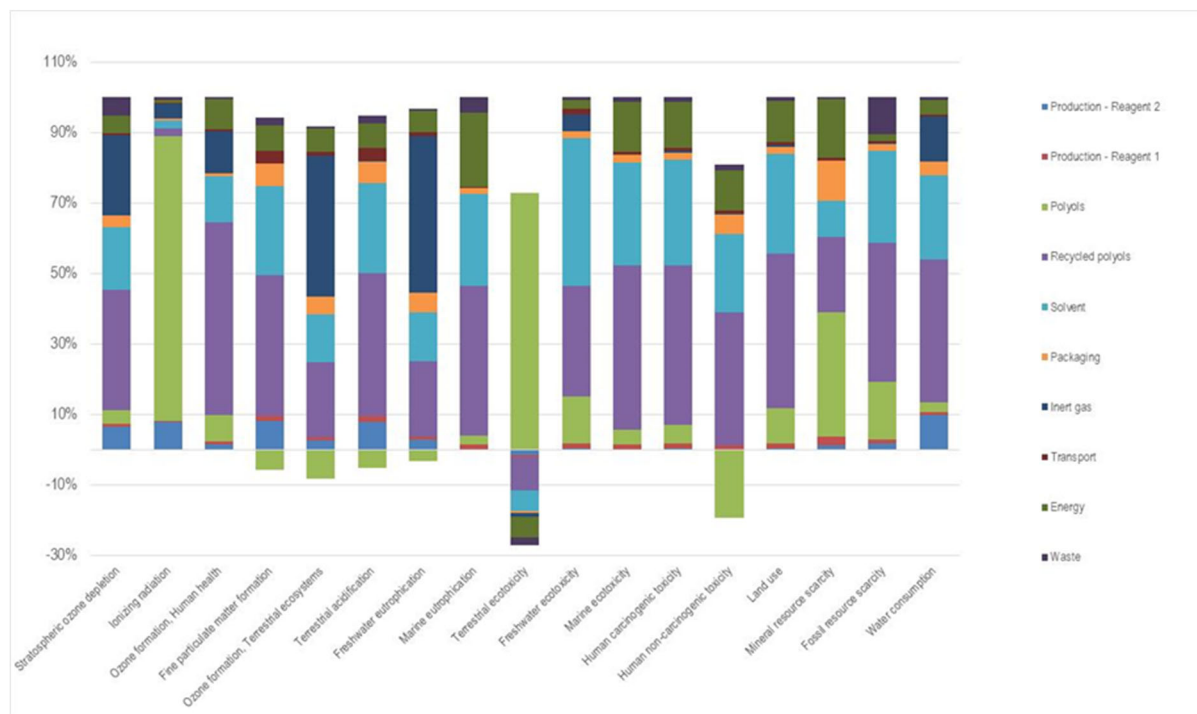
Figure. Results of LCA analysis for 10 kg Rescoll UrbanRec PUR Hot Melt
